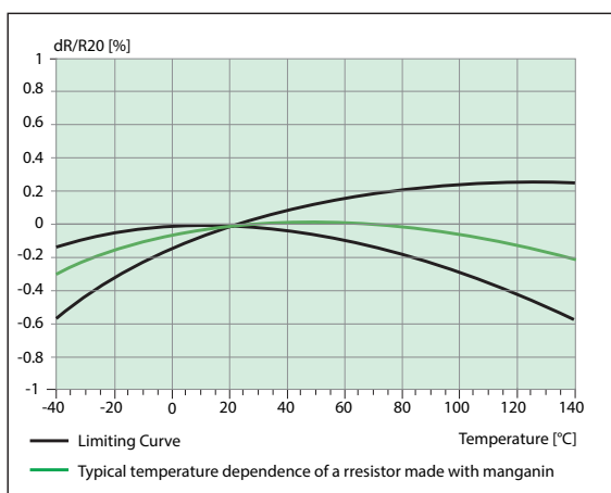
TYPICAL TEMPERATURE DEPENDANCE OF THE ELECTRICAL RESISTANCE
