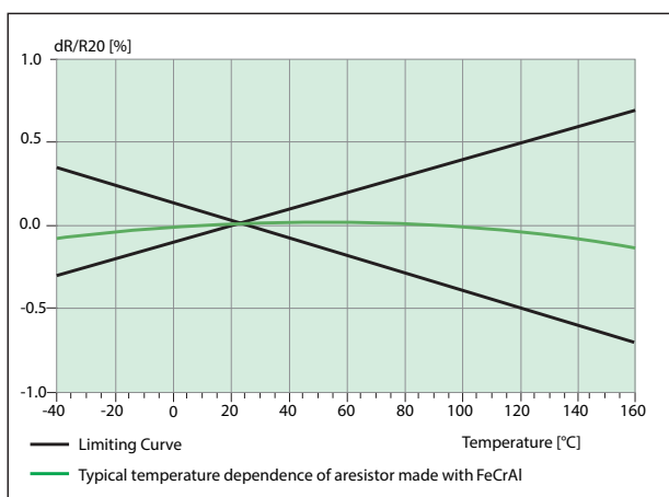
TYPICAL TEMPERATURE DEPENDANCE OF THE ELECTRICAL RESISTANCE
