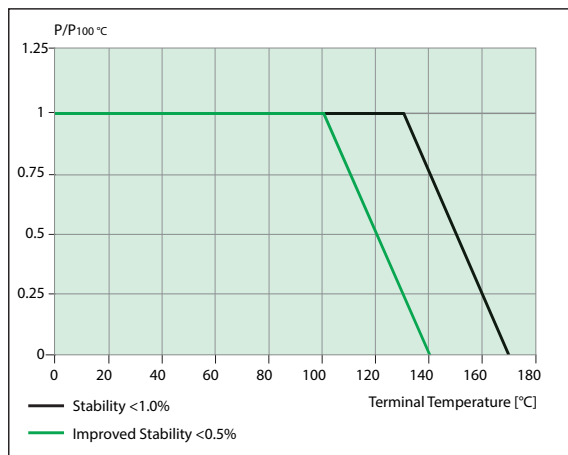
TYPICAL POWER DERATING CURVE FOR RESISTOR WHEN FULL POWER IS AT 100°C & 130°C
