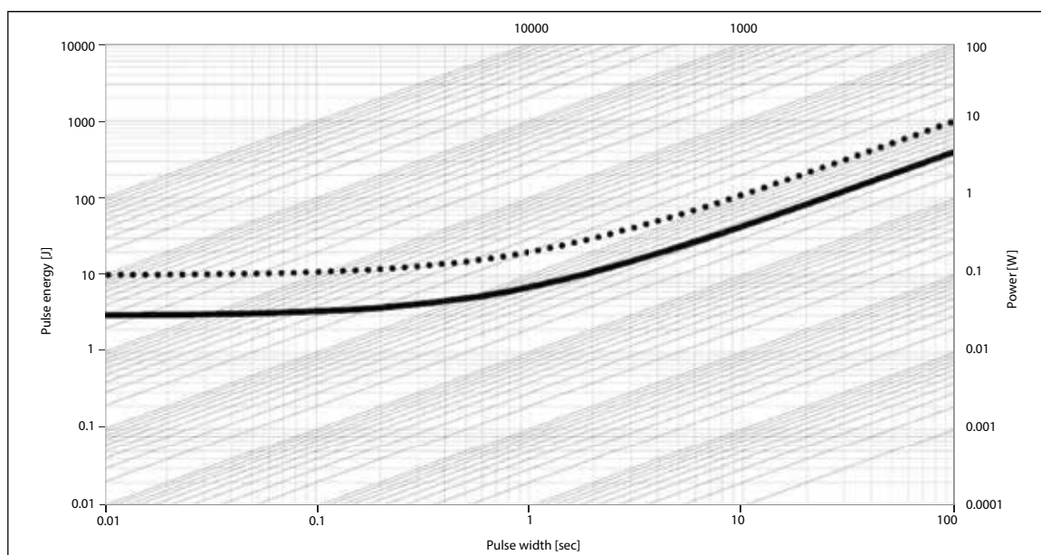
MAXIMUM PULSE ENERGY WITH RESPECT TO PULSE POWER FOR PERMANANT OPERATION
